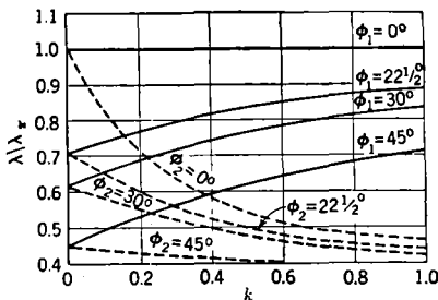
FIG. 4-11.—The dependence of \lambda/\lambda_\tau on k for various values of \phi_1 and \phi_2 in a double-strapped tube. The solid lines are \cos \phi_1 (symmetric modes); the broken lines are \cos \phi_2 (antisymmetric modes).
